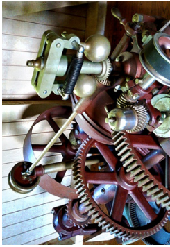
Woodward Size F Governor by Ken Kovar
